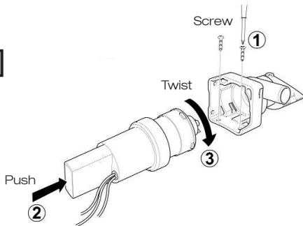
Figure 3- NOTE: Do NOT screw directly onto the hull
